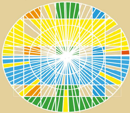
Cells - Xthroughs
