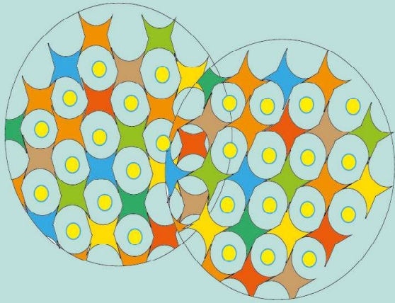
Cells - Constinent
